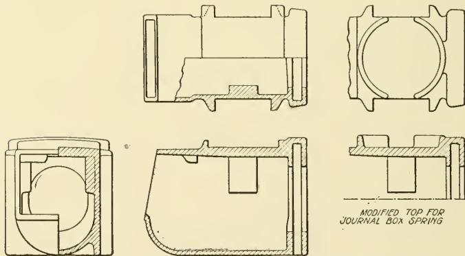
Fig. 17. American Electric Railway Engineering Association Standard Journal Boxes
